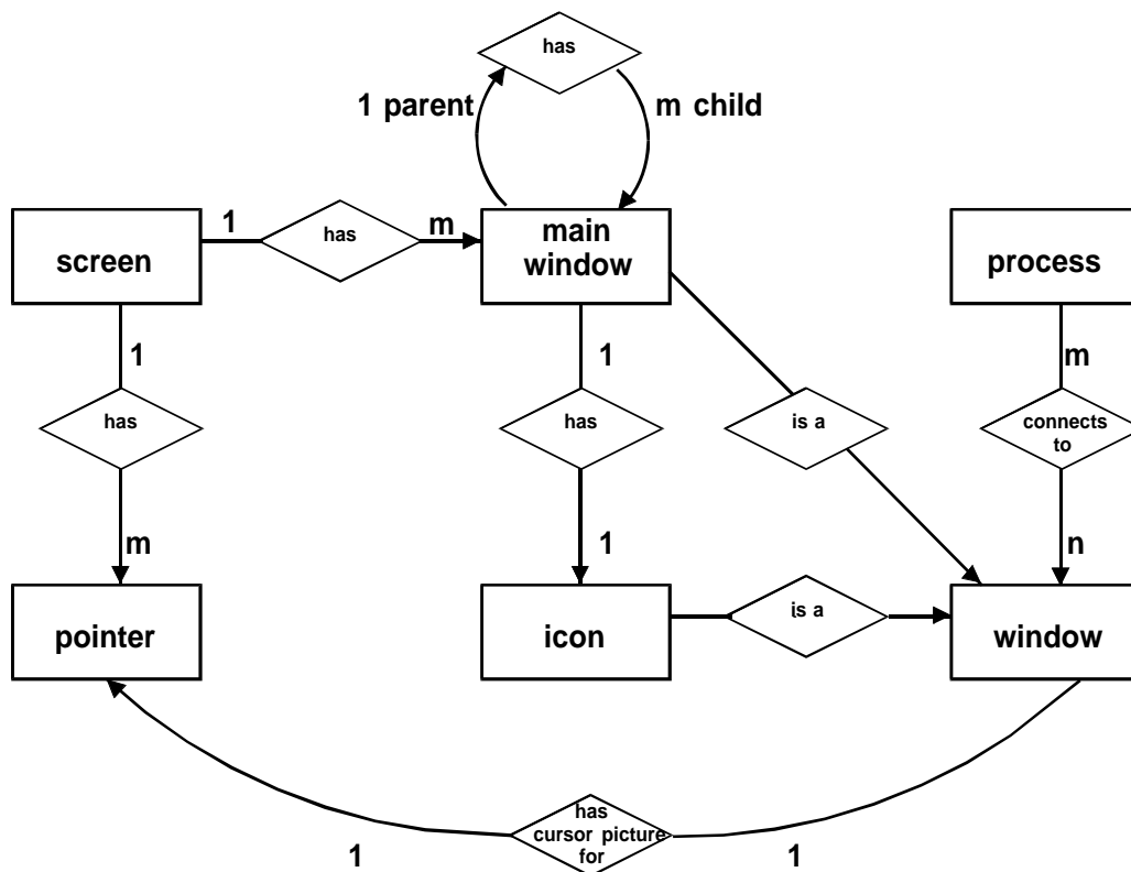
Figure 7-5: Window Manager Entity-Relationship Diagram
