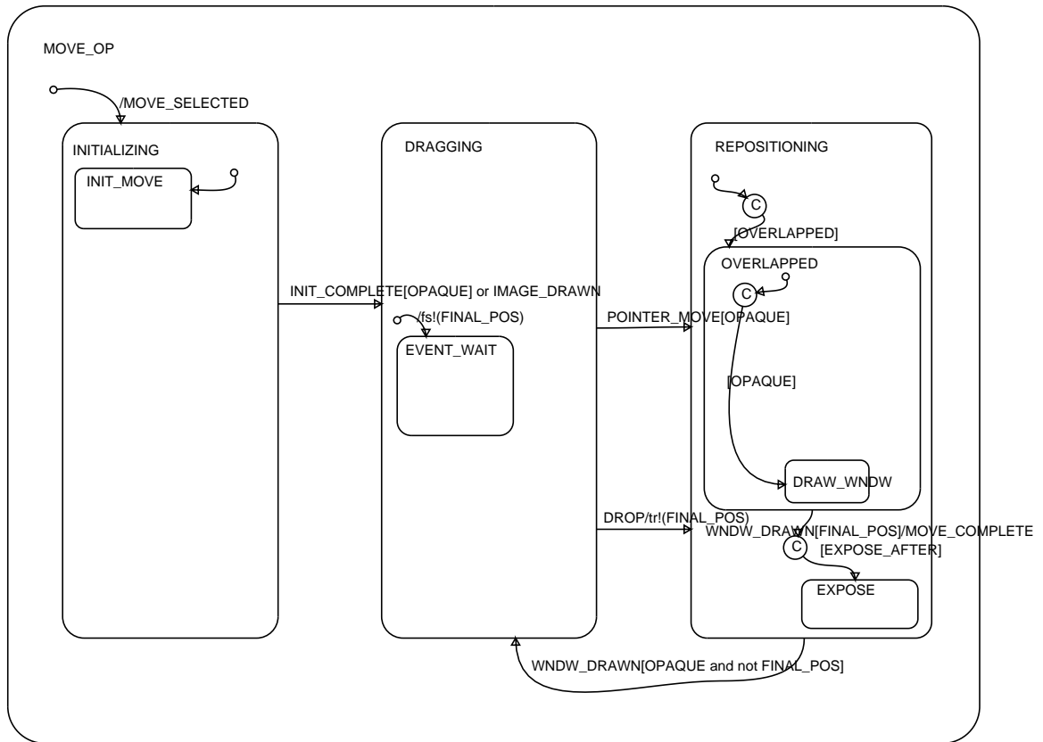
Figure 7-15: Statechart Illustrating X10/uwm Specification
